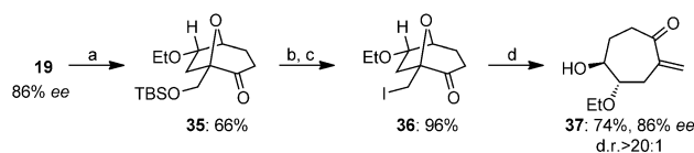
Scheme 5. Stereocontrolled preparation of cycloheptanone 37 . Reaction conditions: a) \text{SiH}_2\text{Ph}_2 , \text{ZnCl}_2 (10 mol %), [\text{Pd}(\text{PPh}_3)_4] (2 mol %), \text{CHCl}_3 ; b) AcOH, HCl, THF, \text{H}_2\text{O} ; c) \text{I}_2 , \text{PPh}_3 , imidazole, \text{C}_6\text{H}_6 ; d) Zn, MeOH.
